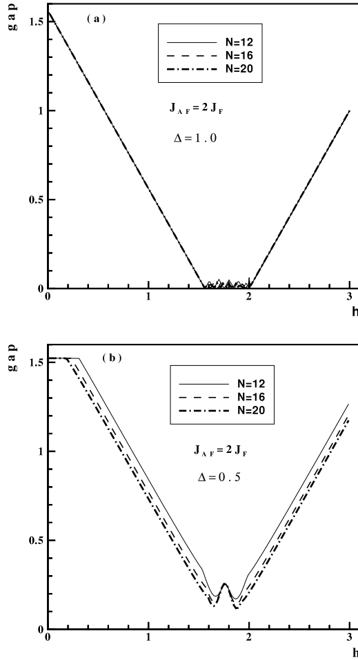
Figure 2. (a) The excitation gap of a spin-1/2 AF-F chain for the isotropic case \Delta = 1.0 in a uniform magnetic field for different size numbers ( N = 12, 16, 20 ). (b) The excitation gap of a spin-1/2 AF-F chain in a uniform transverse magnetic field with anisotropic ferromagnetic coupling \Delta = 0.5 , for different size numbers ( N = 12, 16, 20 ).
