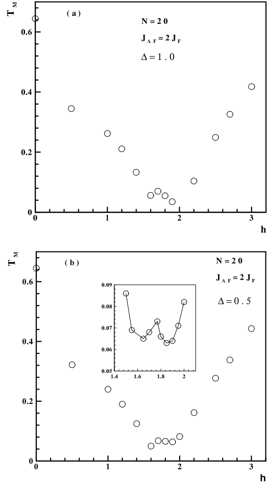
Figure 3. (a) The Schottky heat capacity peak value, T_M , versus the transverse magnetic field, for a spin-1/2 AF-F chain, and the isotropic case \Delta = 1.0 in the uniform transverse magnetic field for system size: N = 20 . (b) The Schottky heat capacity peak value, T_M , as a function of the magnetic field, for a spin-1/2 AF-F chain in the uniform transverse magnetic field with anisotropic ferromagnetic coupling: \Delta = 0.5 , and size number: N = 20 . The inset shows the same quantity in the intermediate magnetic field region, h_{c_1} < h < h_{c_2} .
