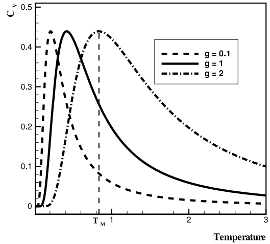
Figure 1. Temperature-dependence of the heat capacity of TLS (equation (5)) for different energy gap values ( g ). T_M shows the position of the Schottky heat capacity peak for the system with g = 2 .
