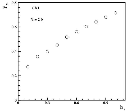
Figure 5. (a) The excitation gap of the 1D AF-Heisenberg model in a staggered field as a function of the magnetic field for different size number ( N = 12, 16, 20 ). (b) The position of the Schottky heat capacity peak, T_M , for the 1D AF-Heisenberg model in a staggered field versus the staggered magnetic field with size number N = 20 .
