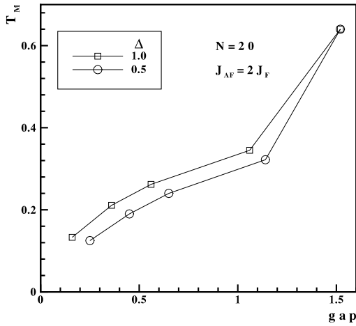
Figure 4. The Schottky heat capacity peak value, T_M , versus the energy gap for a spin-1/2 AF-F chain with anisotropic ferromagnetic couplings: \Delta = 1.0 and \Delta = 0.5 , and size number: N = 20 .
